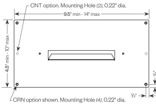
Front Mount Plate (FMP-PRCD8)
