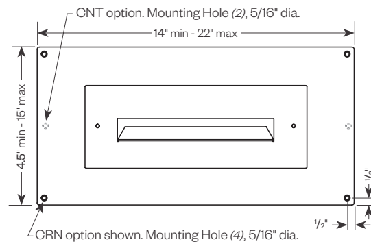
Rear Mount Plate ( RMP-PRC12 )
