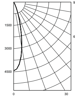
Flood (FL) Distribution, 28° LTL #818201 Lumens: 958
