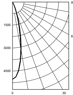
Medium Flood (MFL) Distribution, 25° LTL #818200 Lumens: 1,010
