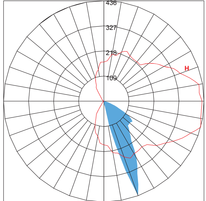
AB5 34" 180° Polar Graph (shown with optional GS)
