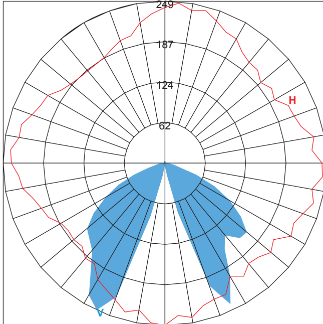
AB5 34" 360° Polar Graph
