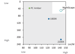
Blue radiation per lumen
