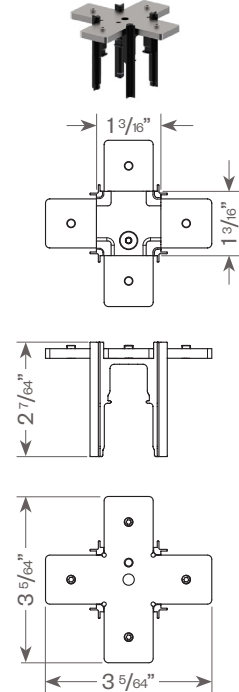
X - Joint
