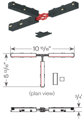
Polarized T Feed (Internal Left)
