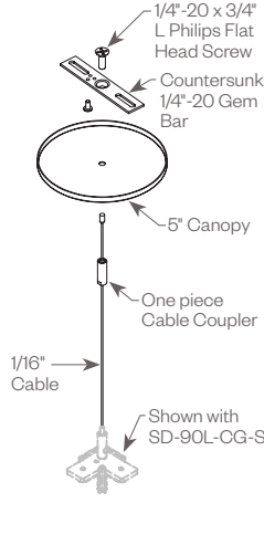
Non-Power Feed (when suspending to L, T, X Connector with cable gripper)
