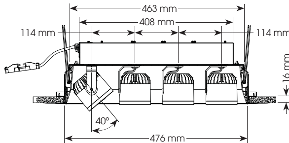
Ceiling Cut Out Dimension: 141 mm x 491 mm
