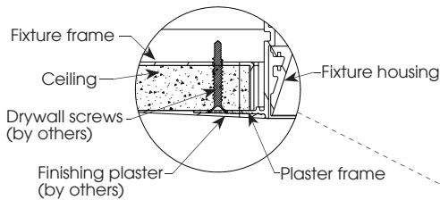
Ceiling Cut Out Dimension: 141 mm x 491 mm
