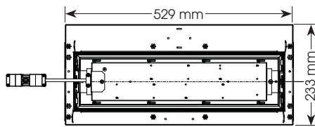
Ceiling Cut Out Dimension: 141 mm x 491 mm
