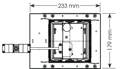
Ceiling Cut Out Dimension: 141 mm x 141 mm
