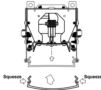
3. Secure reflector to upper area of extrusion via 8-32 screws. 4. Install lens. Starting at (1) end, squeeze lens legs IN to snap LENS in place, and continue pressing upwards across the length of the fixture until lens is secure.
