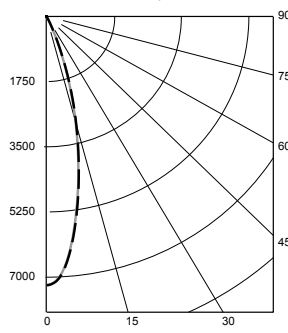
Flood (FL) Distribution, 25° LTL # 13663493.16 Lumens: 1584; lm/W: 93.9
