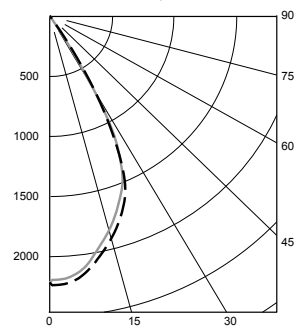
Very Wide Flood (VWF) Distribution, 55° LTL # 13663493.18 Lumens: 1558; lm/W: 92.8
