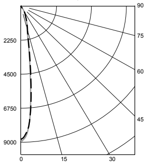
Spot (SP) Distribution, 15° LTL # 13663493.15 Lumens: 1505; lm/W: 89.5
