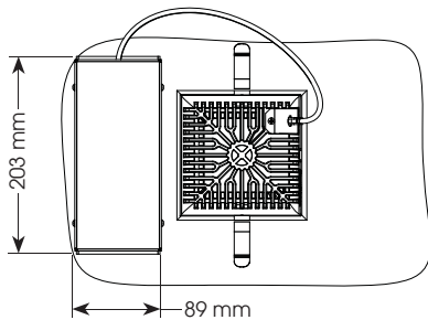
Ceiling Cut Out Dimension: 133 mm sq.
