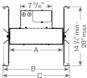
Hanger Bar Mounted on End of Housing
