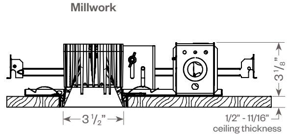
Millwork Ceiling cut out: 4" sq.
