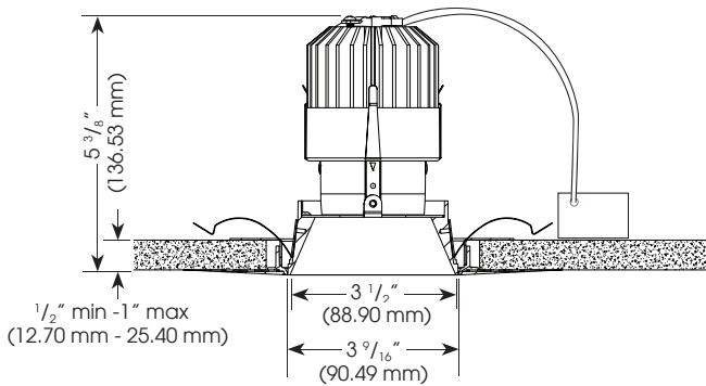
Ceiling Cut Out Dimension: 4 1/2" (114.3 mm)
