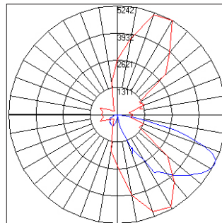
DS323FC-3M-30-T3-600M
