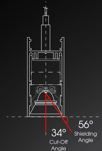
Figure 1 – Shielding & Cut-Off Angles
